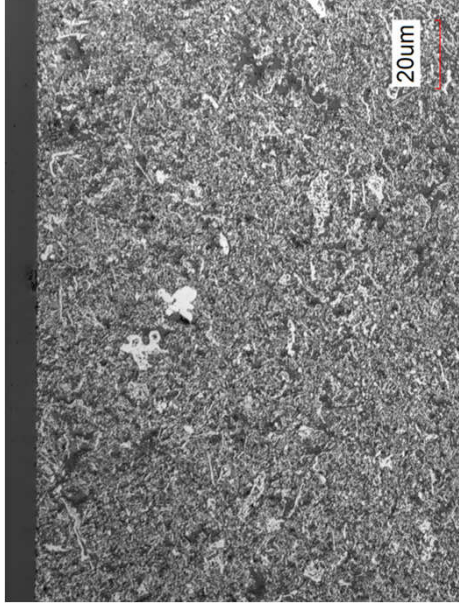
As sintered (900 °C, 5K/min, 3h, air)
